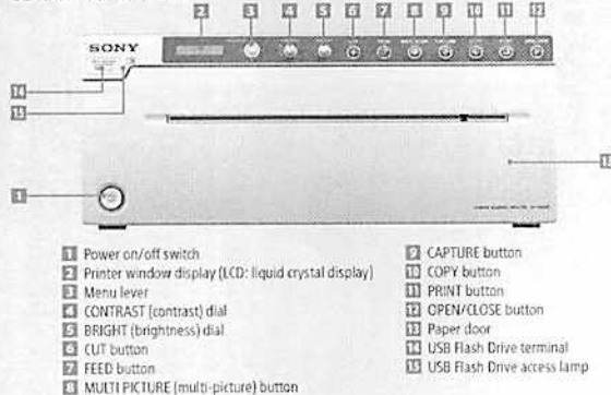
UP-971AD Front Panel
