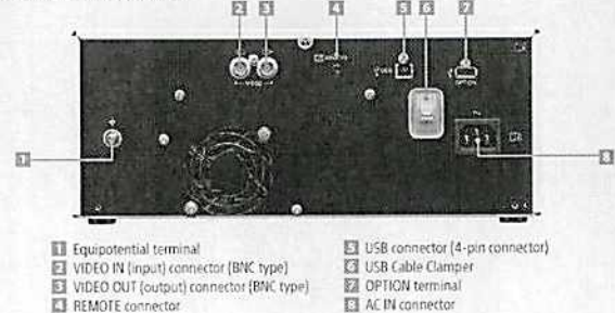
UP-991AD Rear Panel
