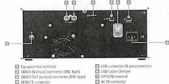
UP-971AD Rear Panel
